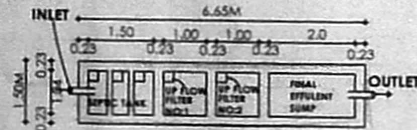
DETAILS OF SPTIC TANK WITH UP FLOW FILTERS
